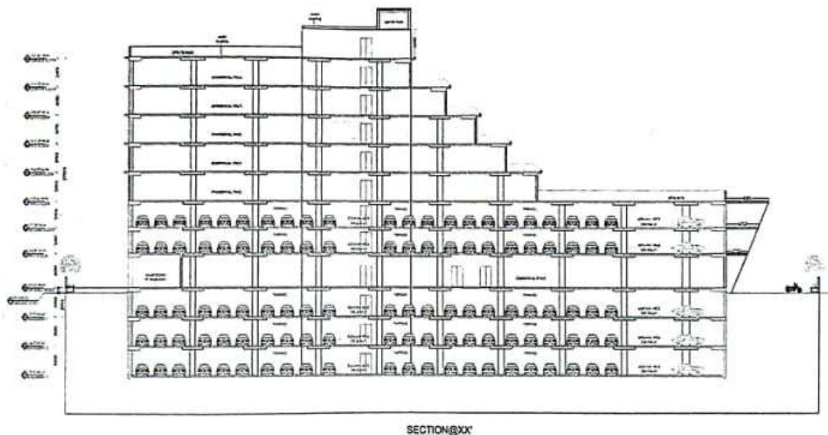
SECTION XX'
